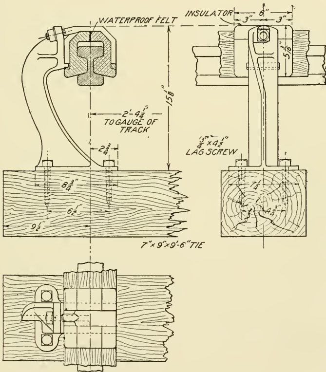
Fig. 202. Details of Insulator and Bracket for Inverted Rail
